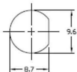
RECOMMENDED MOUNTING HOLE DIM'S
